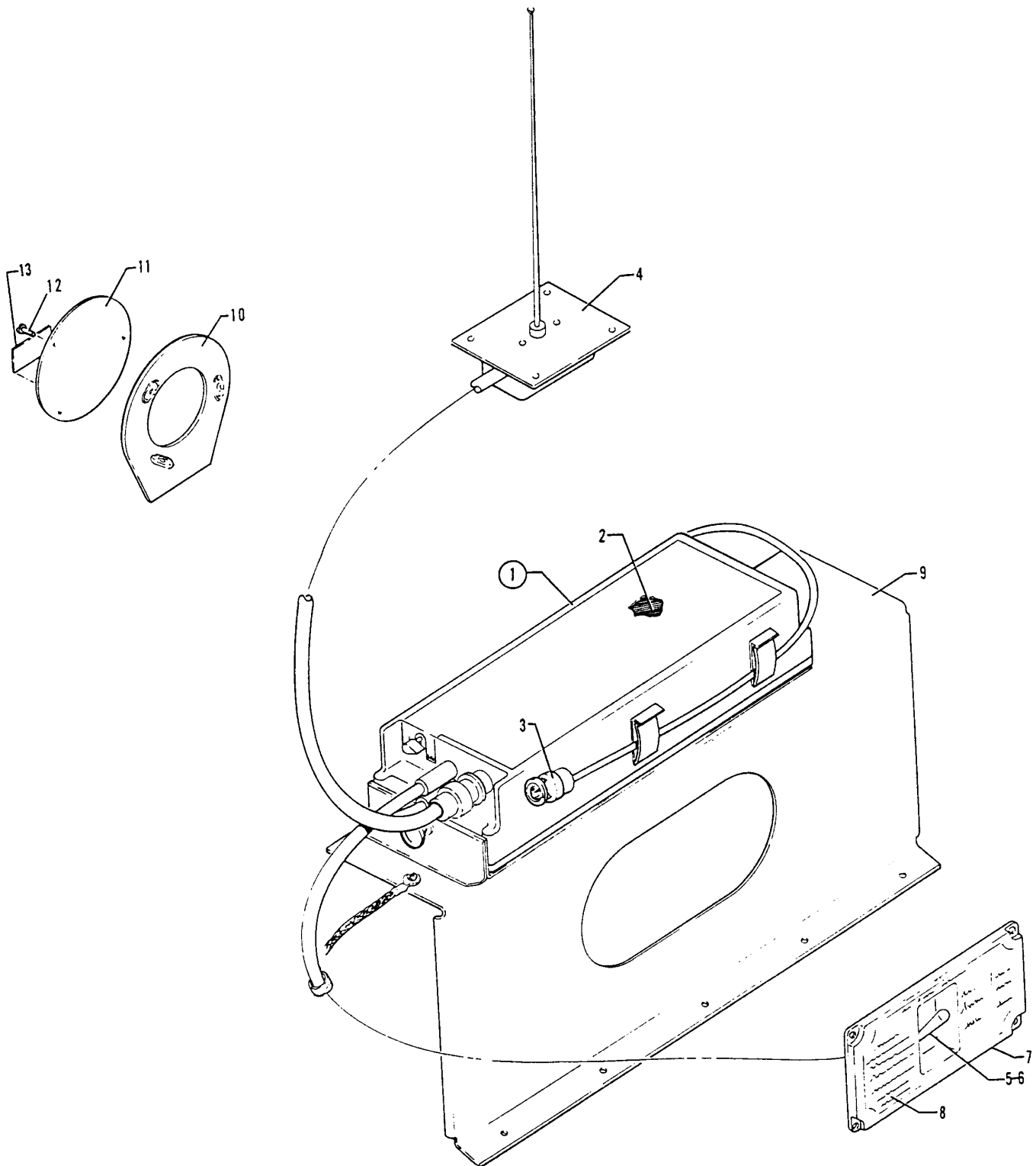
Figure 76. Piper Automatic Locator (ELT) Installation (Communications Components Corp.)
