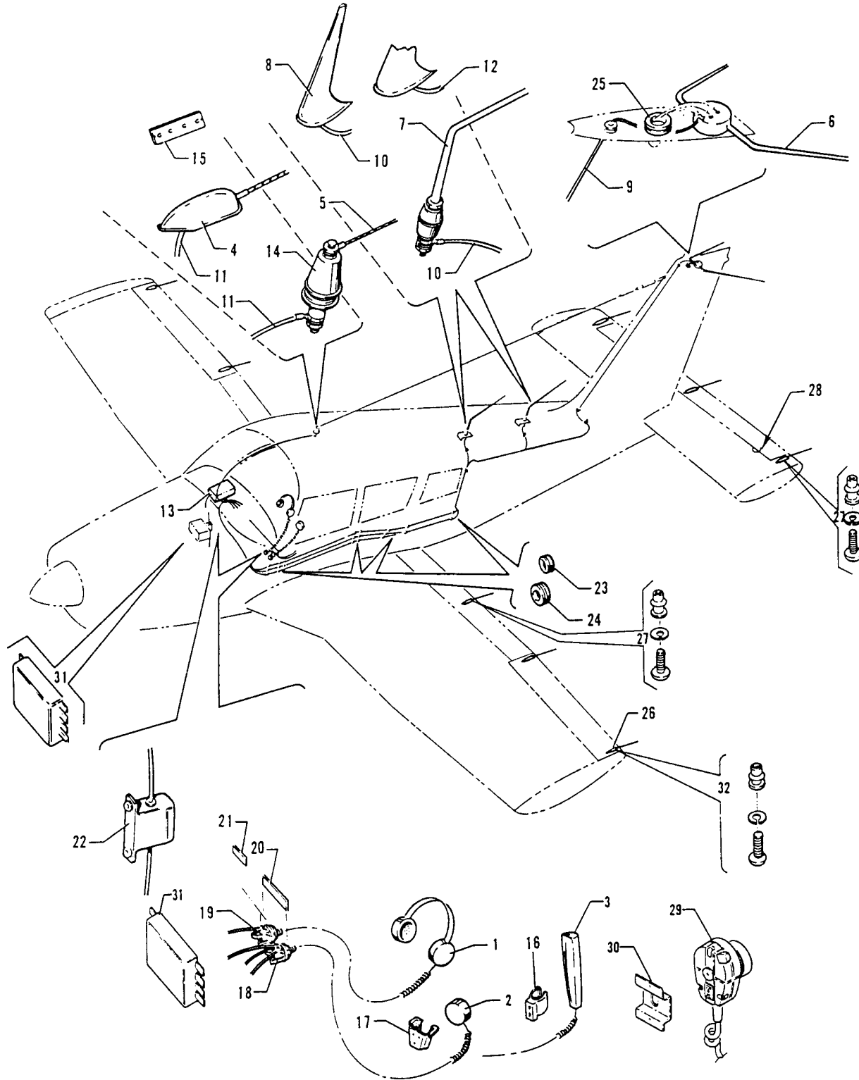
Figure 79. Radio, Antenna System and Static Wicks Installation
