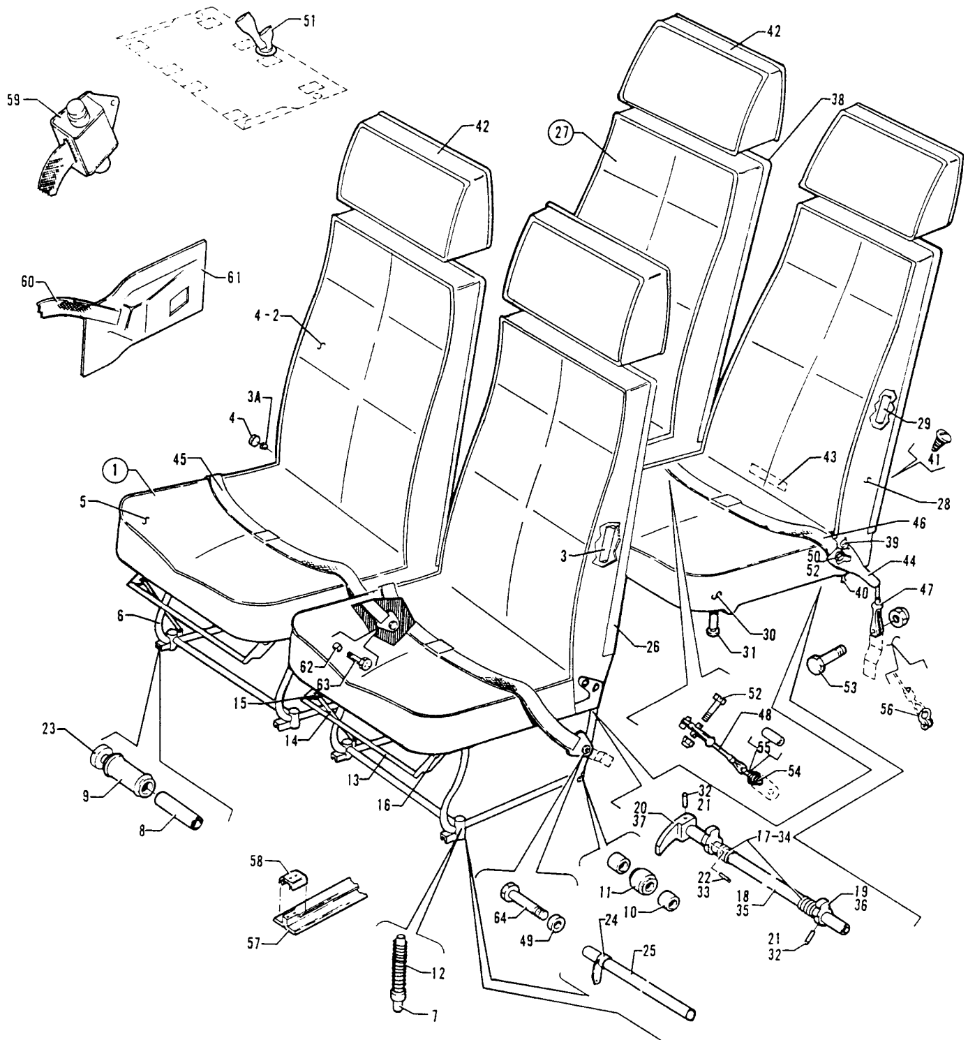
Figure 33. Seats Installation
