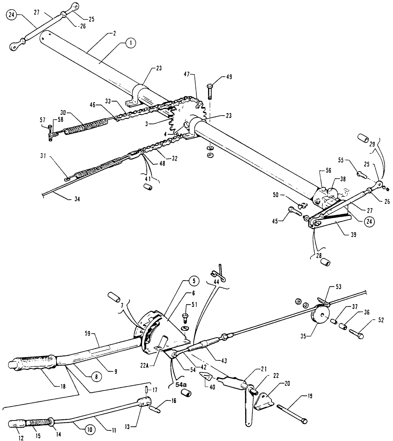
Figure 54. Flap Control Installation
