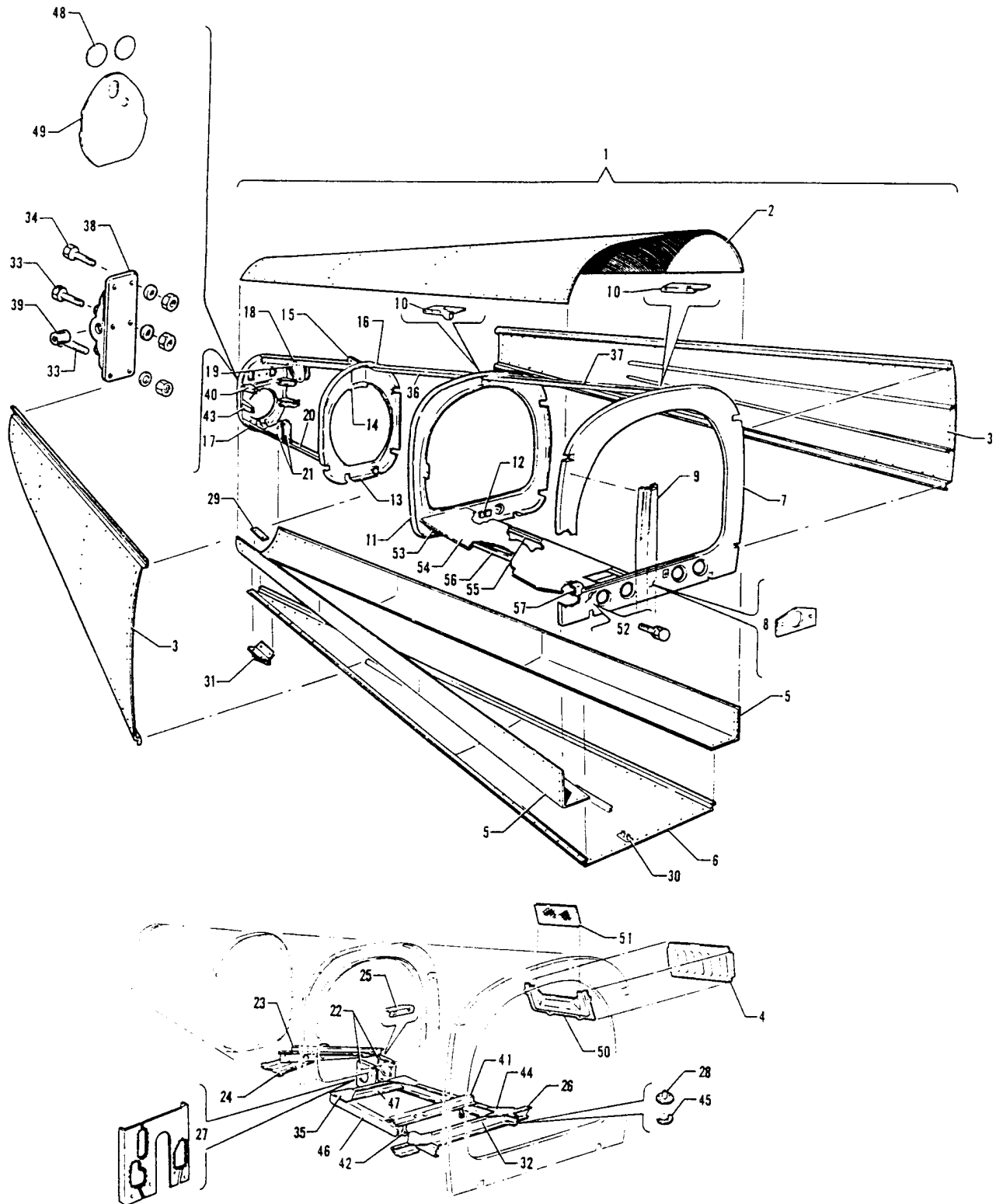
Figure 12. Fuselage Aft Section
