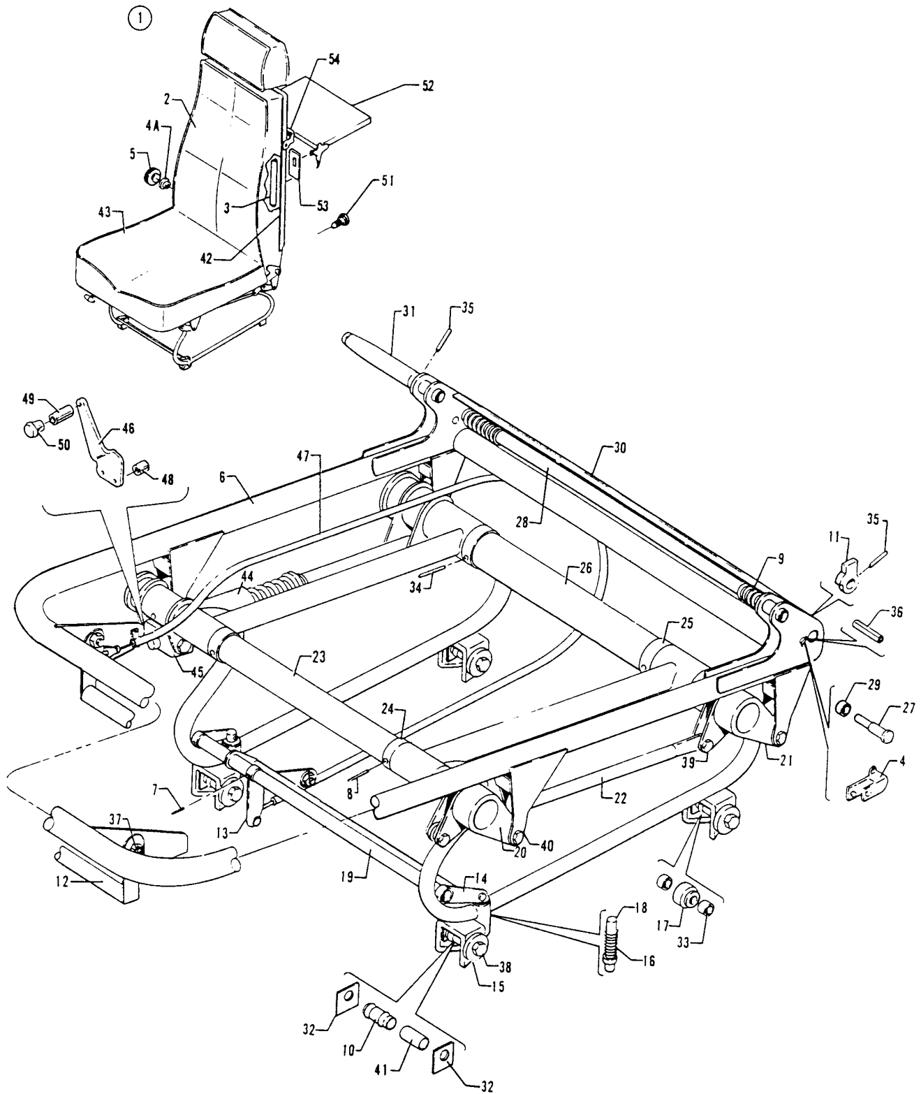
Figure 34. Vertically Adjustable Front Seat Assembly
