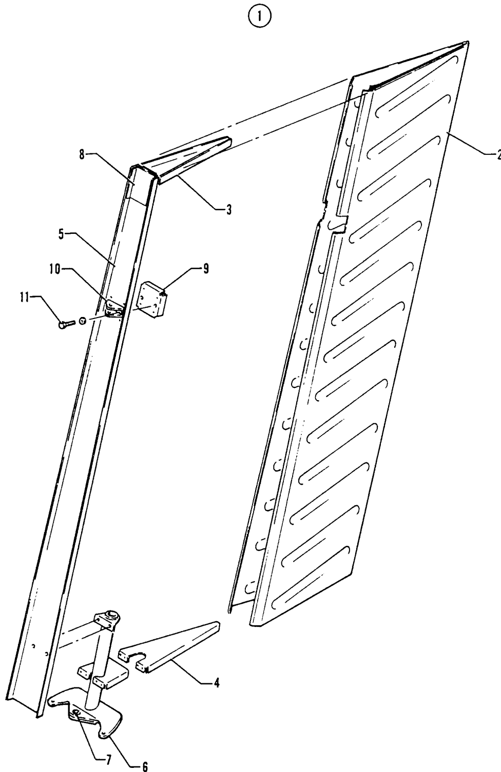
Figure 18. Rudder Assembly
