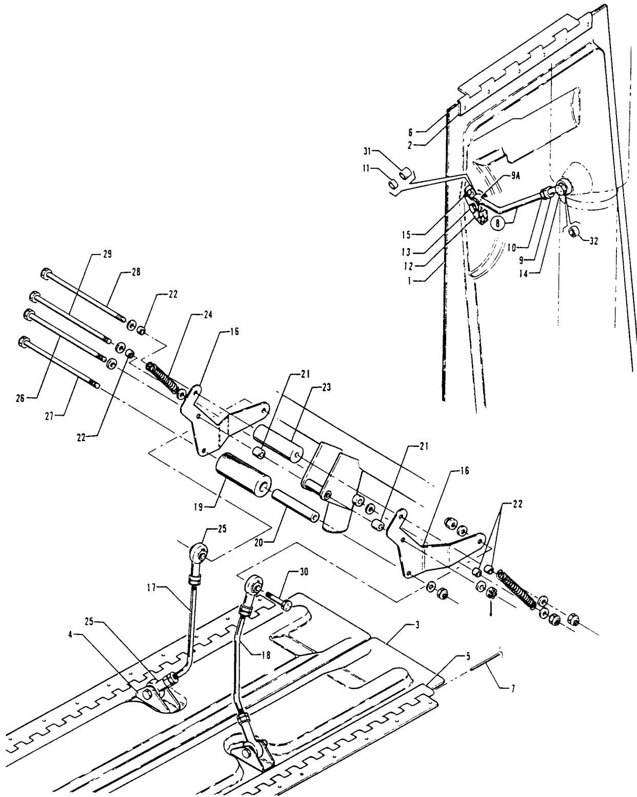
Figure 27. Landing Gear Door Installation (PA-28R-201T)
