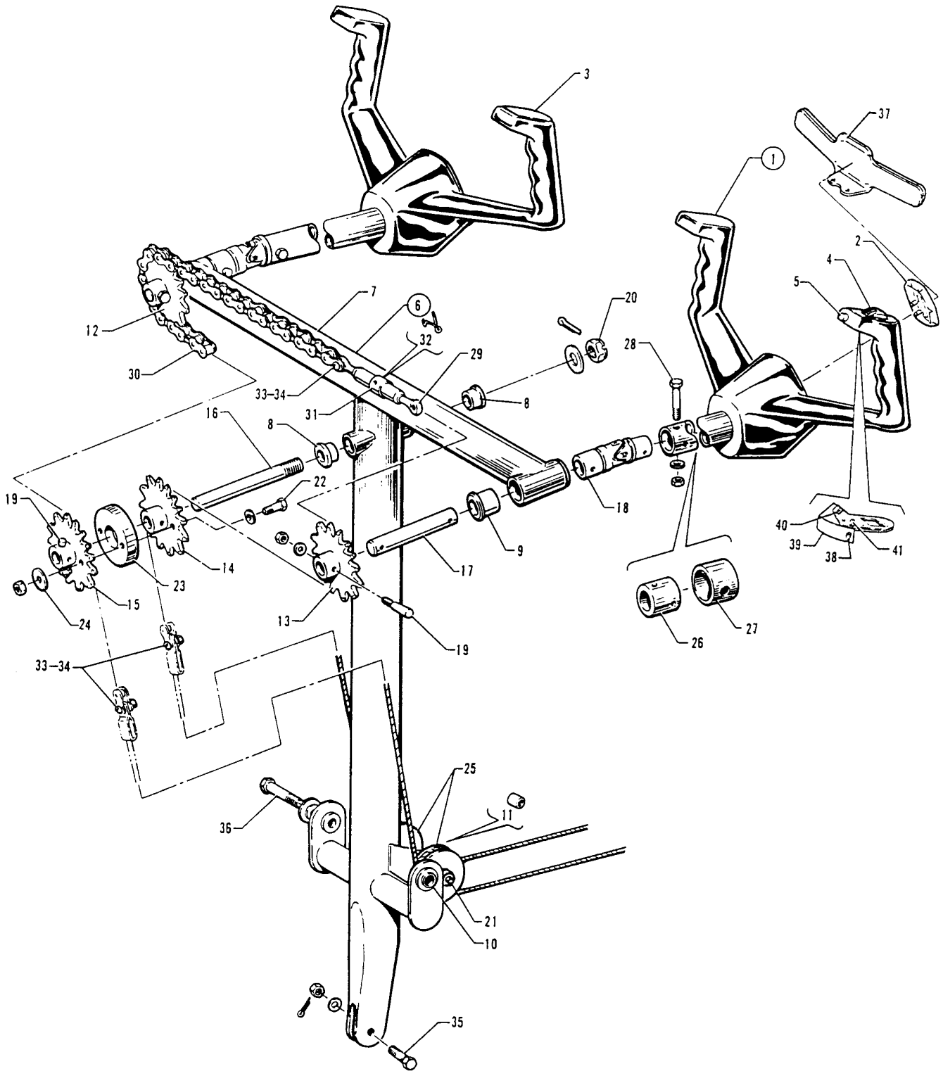
Figure 57. Control Wheel Installation
