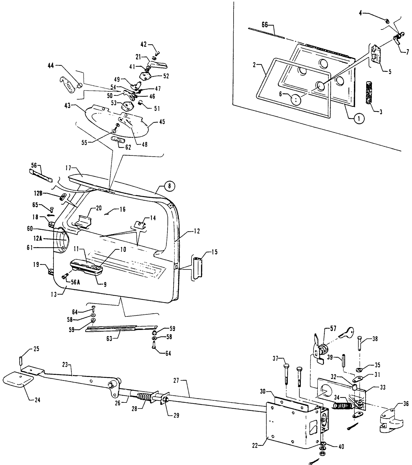
Figure 13. Fuselage Cabin and Baggage Door Installation
