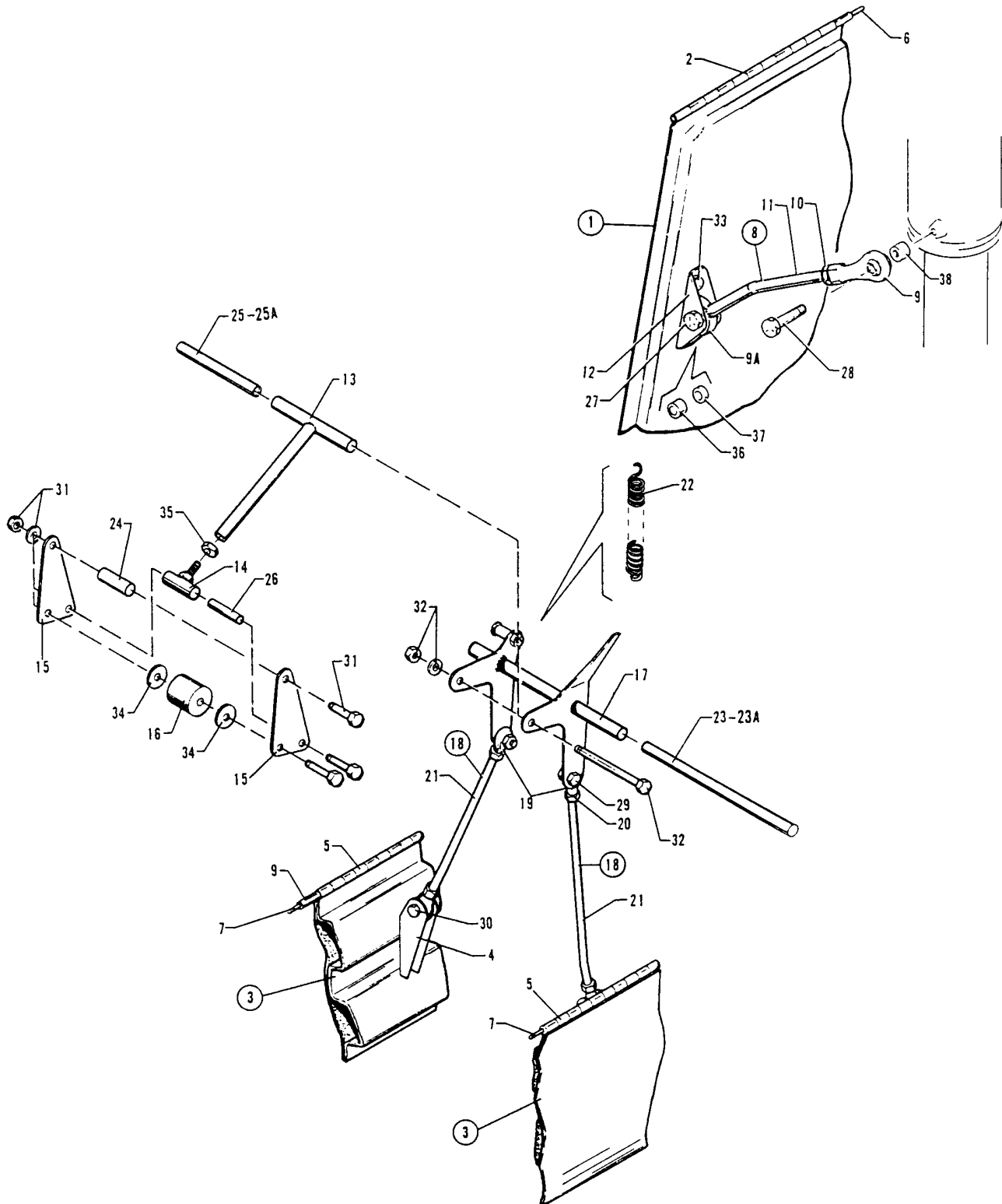
Figure 26. Landing Gear Door Installation (PA-28R-201)
