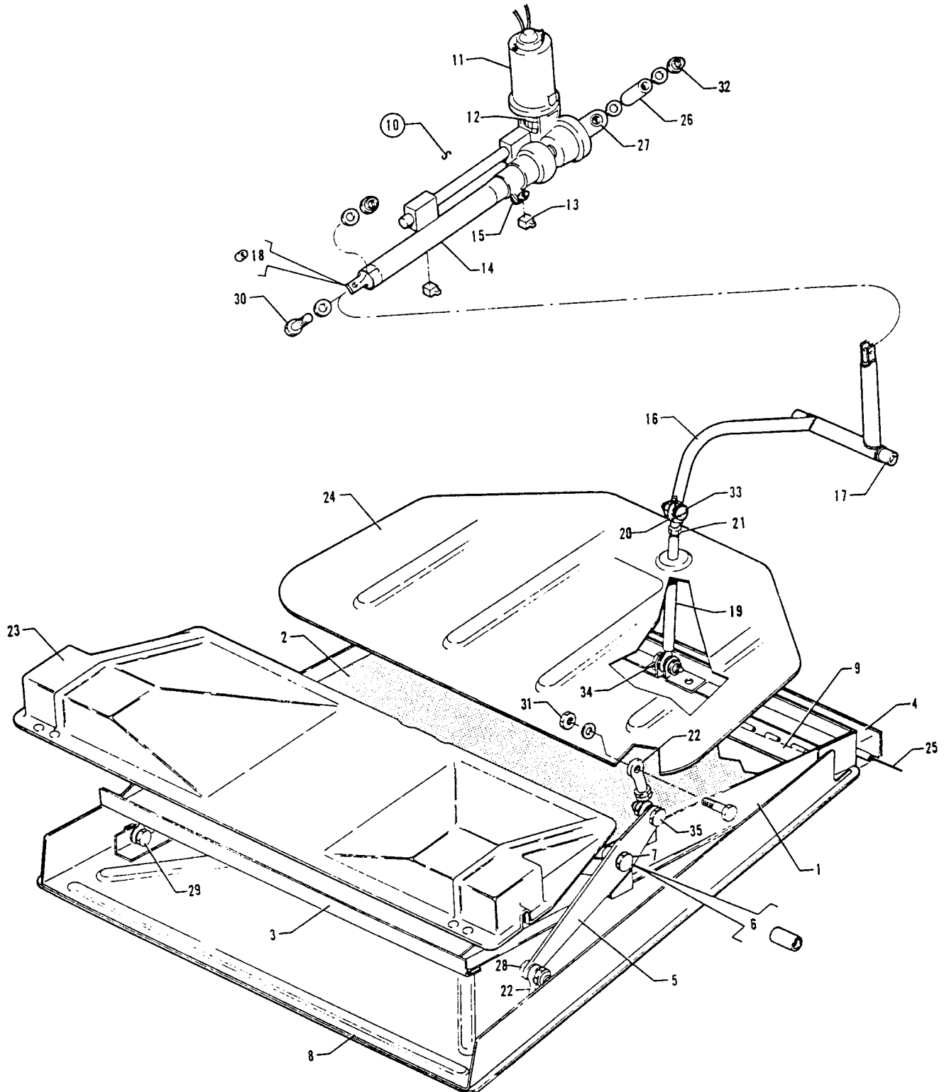
Figure 66. Air Conditioner Condenser Installation
