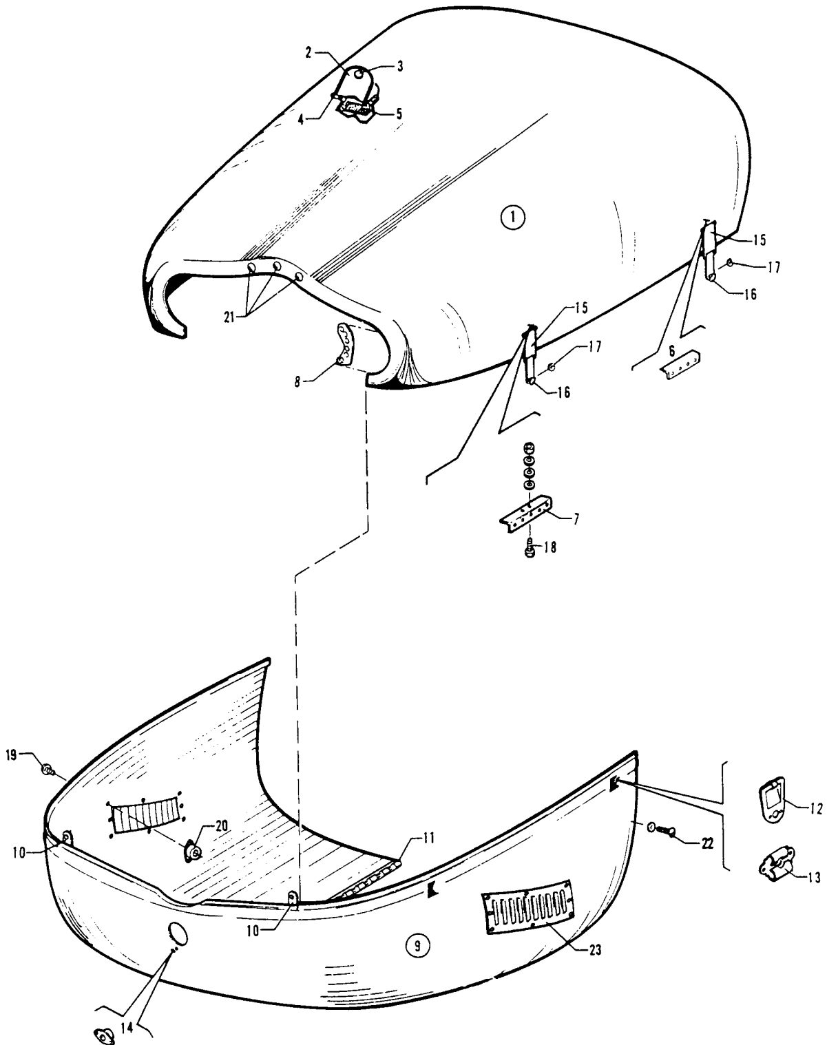
Figure 44. Engine Cowl Installation (PA-28R-201)
