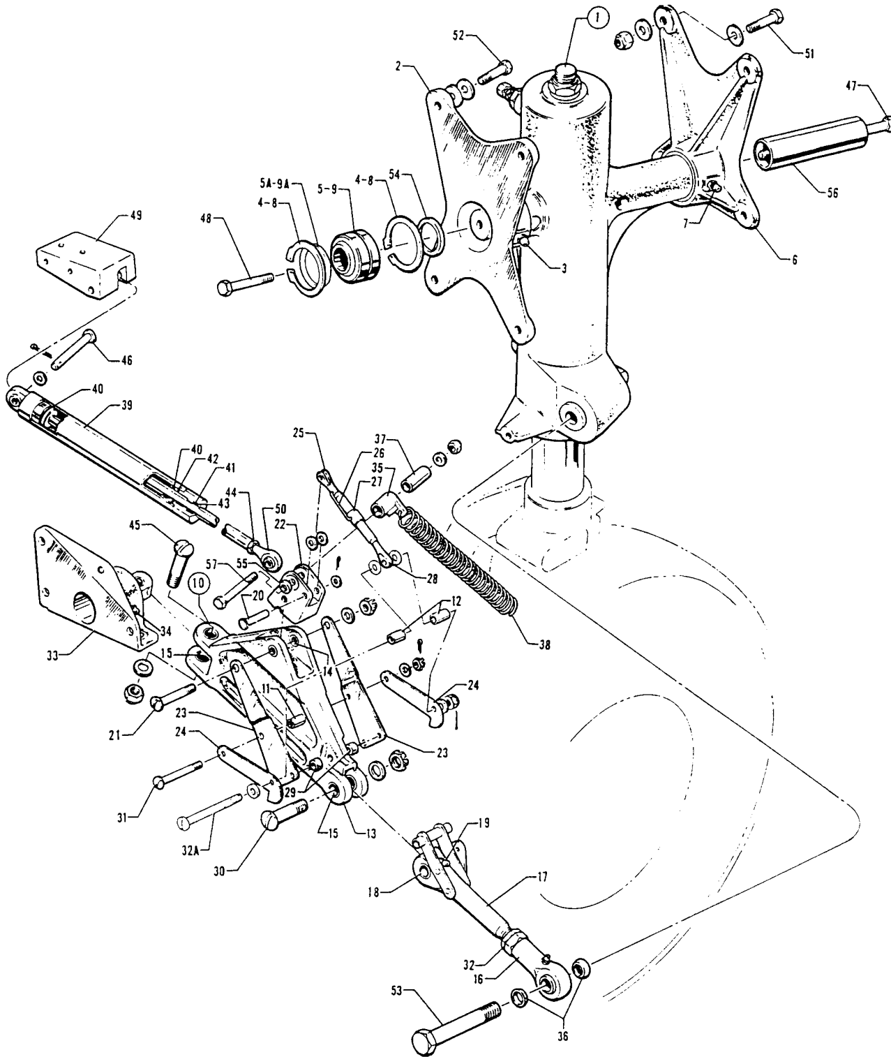
Figure 22. Main Landing Gear Installation
