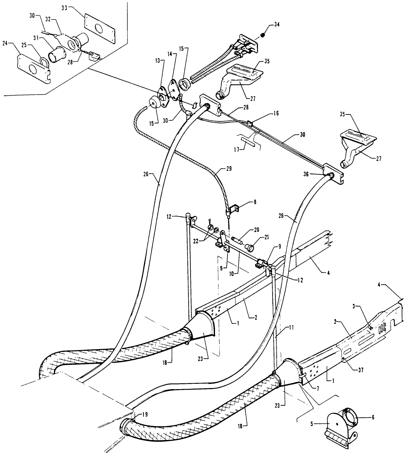
Figure 60. Heat and Defrost System Installation (PA-28R-201)
