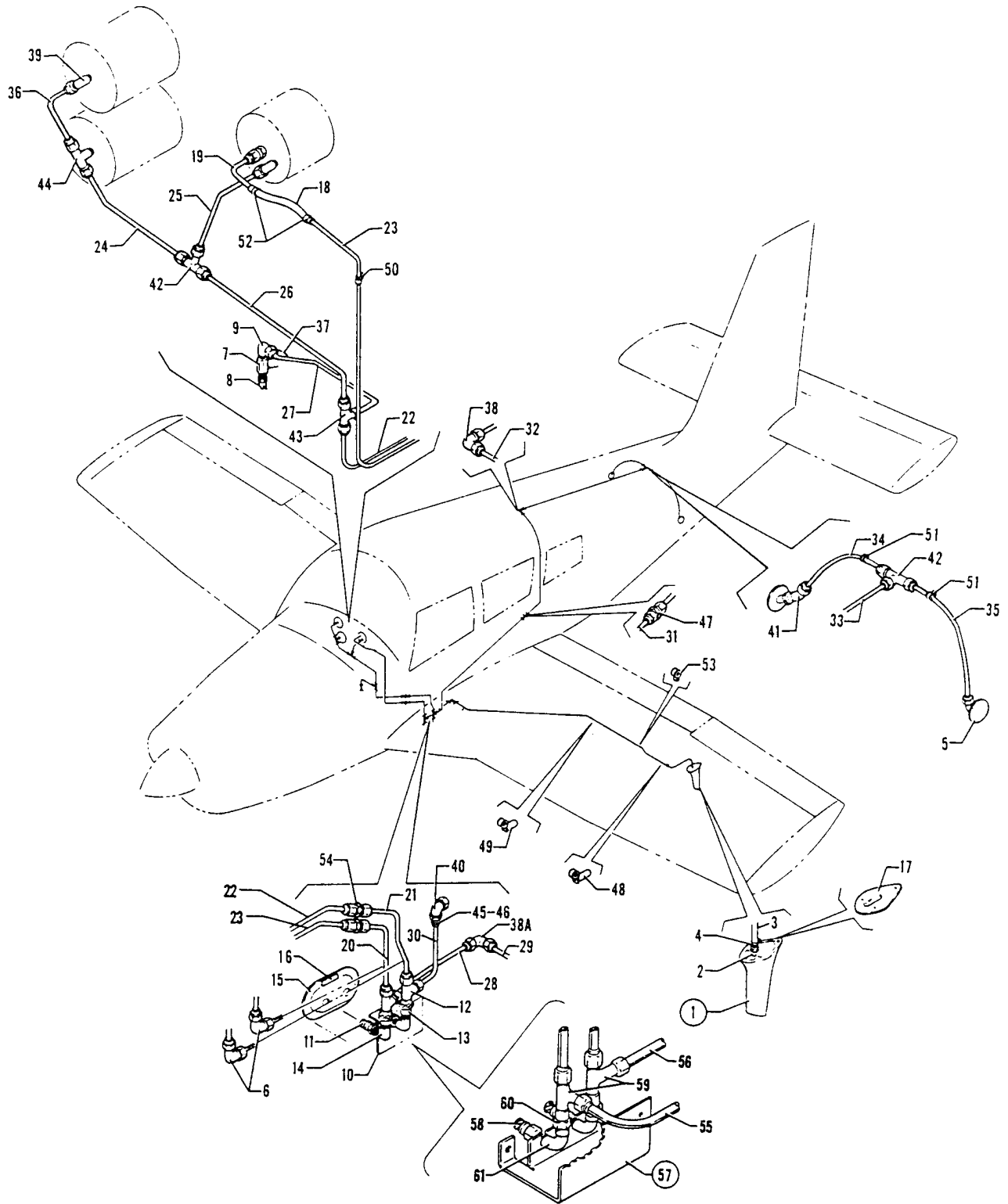
Figure 37. Pitot Static System Installation
