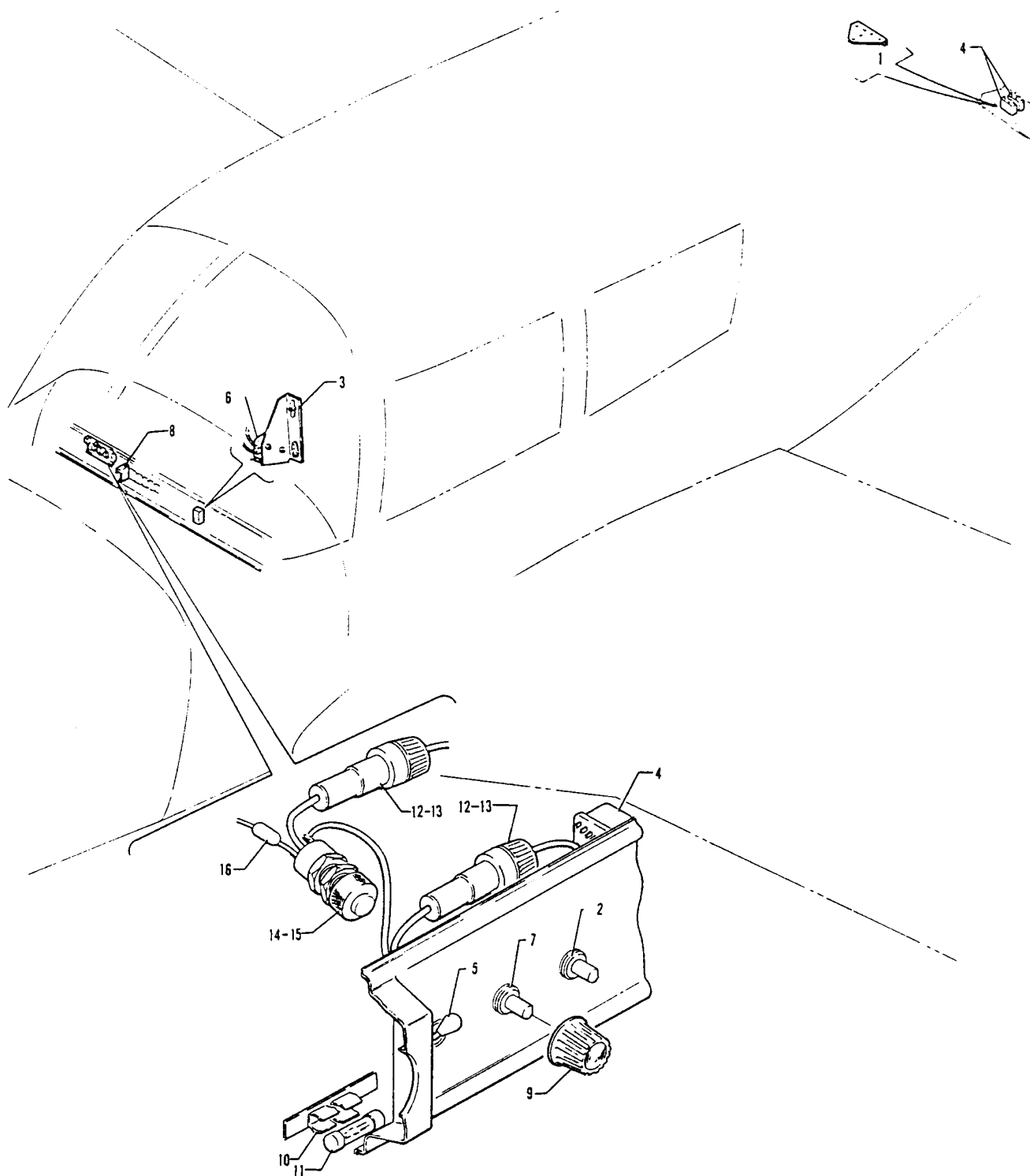
Figure 69. Air Conditioning Electrical Installation
