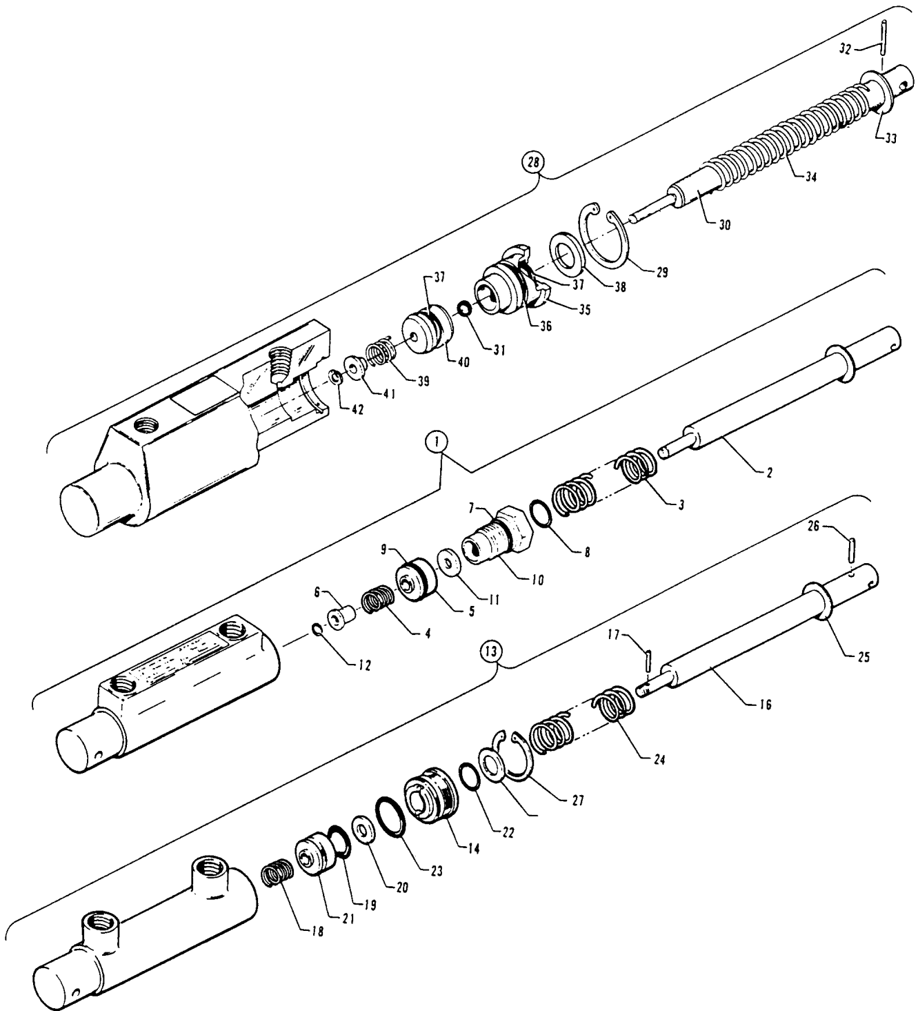
Figure 30. Toe Brake Master Cylinder Assembly
